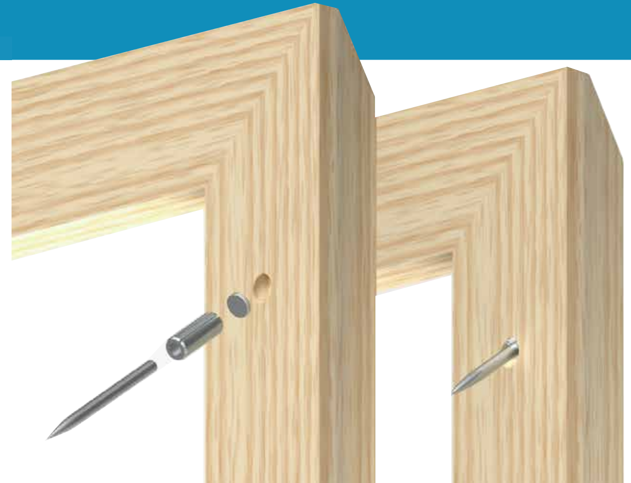
STEP 2 Insert Magnet(s) and Spring Pin(s)
